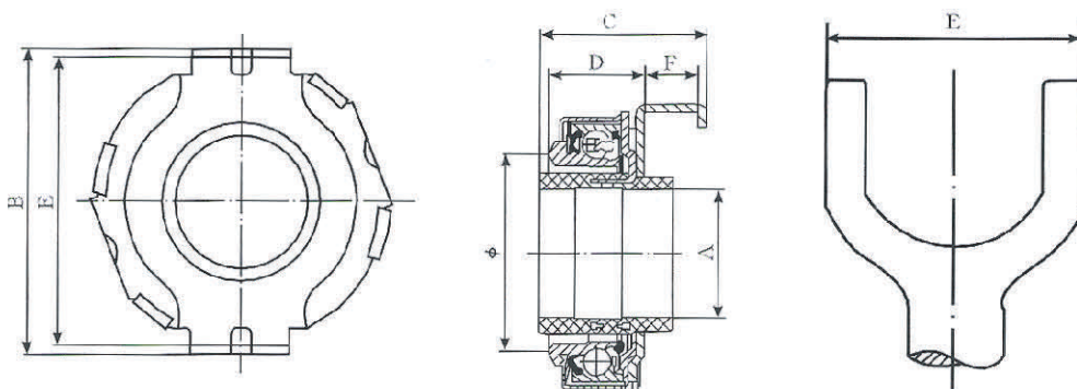
分离面为曲面的外拨叉用自调心分离轴承总成 Self-Centering Release Bearing Assemblies
